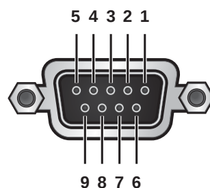
(Rysunek 5-3: Port RS232)
