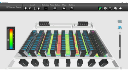
• Data center 3D visualized layout
